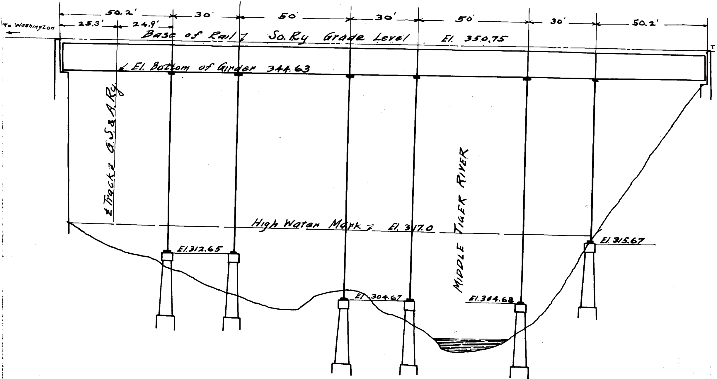
PROFILE ON SOUTHERN RY CENTER LINE Scales 1" = 10' Vert. 1" = 25' Hor.
