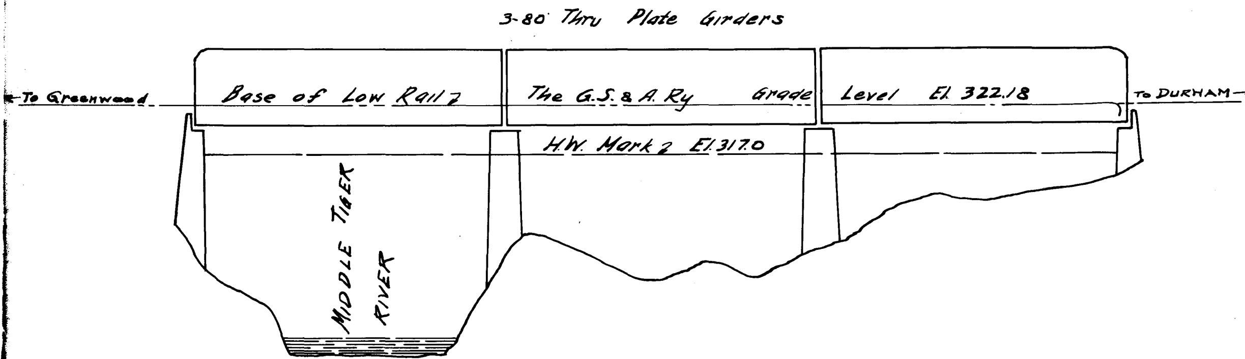
PROFILE ON G. S. & A. RY CENTER LINE Scales 1" = 10' Vert. 1" = 25' Hor.
