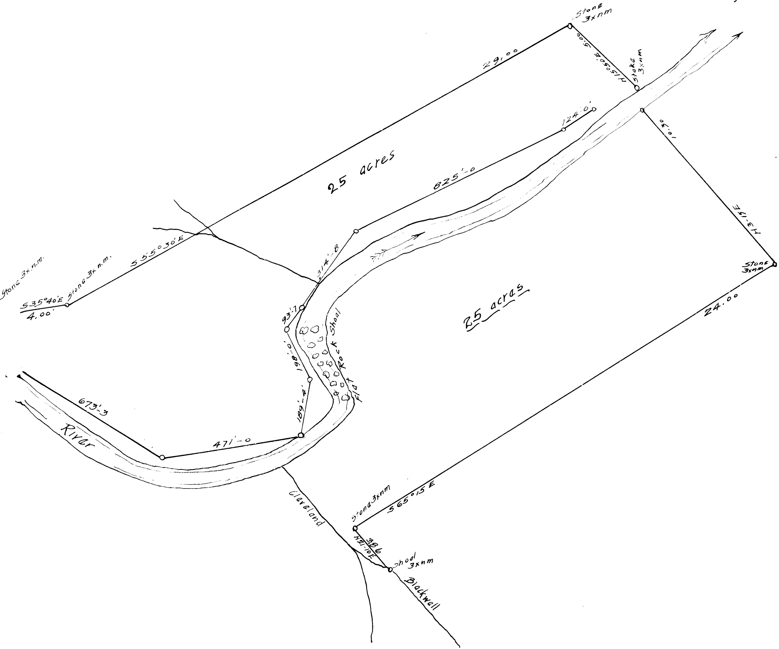
Map of Flowaga Areas above Flat Rock Shoals - Pacolet River Spartanburg Co, S. C. - Surveyed for Mr. J. B. Cleveland by Kadshaw & Kadshaw-Engrs & Suijrs. Scale 200' to 1" June 16, 05'
